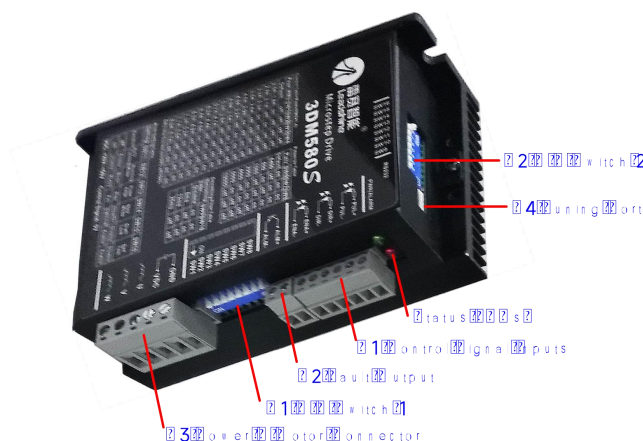
Figure 2 Connectors, DIP switches, and LED locations
